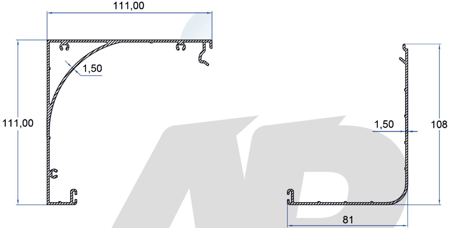
MOTOR KUTUSU ENGINE BOX 2878 1.585 kg/m
